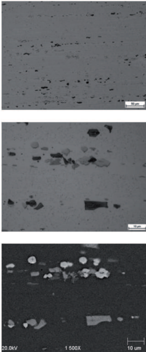
Fig. 9. Microstructures of T6 extrusions from 2014 high alloyed (B alloy)
