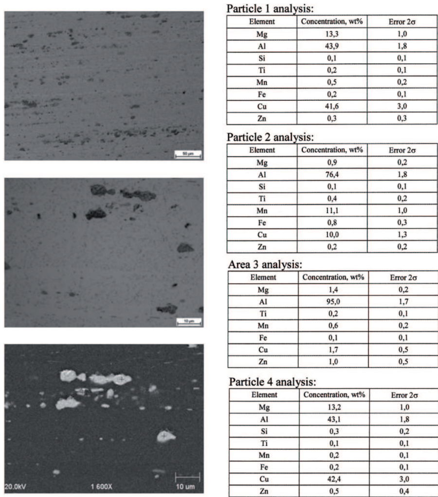
Fig. 11. Microstructures of T6 extrusions from 2024 high alloyed (D alloy)
