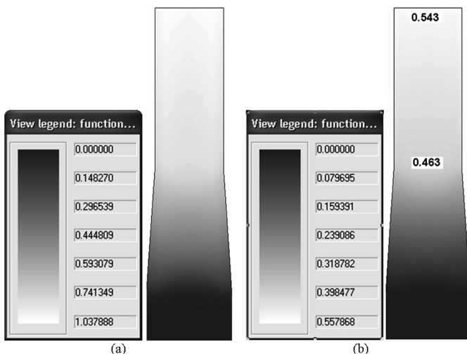
Fig. 5. Results of numerical simulation of drawing process for initial diameter 0.5 mm and final diameter 0.4 mm (elongation 1.56), drawing angle 4°, drawing velocity 0.05 m/s for MgCa0.8. Distribution of: (a) ductility function; (b) effective strain
