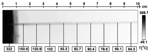
Fig. 1. Distribution of temperature in wire after deformation, obtained by the infrared camera
