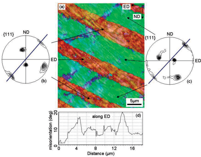
Fig. 6. Details of microstructural and textural changes in the areas of MSB left . (a) Orientation map, and (b) and (c) the {111} pole figures showing textures of particular grains. (d) Misorientation line scan along ED, typically observed in both groups of grains. SEM/EBSD measurements with step size of 100 nm. ND-ED section. ‘IPF (||Y)’ color code was applied
