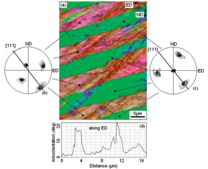
Fig. 7. Details of microstructural and textural changes in the areas of MSB right . (a) Orientation map, and (b) and (c) the {111} pole figures showing textures of particular grains. (d) Misorientation line scan along ED, typically observed in both groups of grains. SEM/EBSD measurements with step size of 100 nm. ND-ED section. ‘IPF (||Z)’ color code was applied
