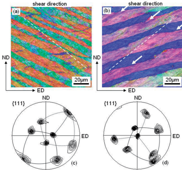
Fig. 5. Microstructural and textural changes in areas of macroscopic shear bands showing opposite tendency of crystal lattice rotation. Orientation maps and corresponding {111} pole figures in areas of: (a) and (c) – MSB left , (b) and (d) – MSB right . SEM/EBSD measurements with step size of 100 nm. ND-ED section. ‘IPF (||Y)’ color code was applied
