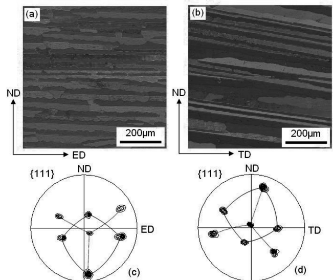
Fig. 1. Microstructure and texture of feathery grains in Al-0.23wt.% alloy after unidirectional solidification. Orientation maps and corresponding \{111\} pole figures measured in: (a) and (c) ND-ED section, (b) and (d) ND-TD section. 'All Euler' color code was applied. SEM/EBSD measurements with step size of 2 \mu\text{m}
