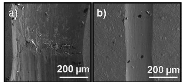
Fig. 12. SEM images of surface of Ni-Mo coatings electrodeposited at current density: a) 1.5 A/dm 2 and b) 5 A/dm 2 after a ball-on-disk test
