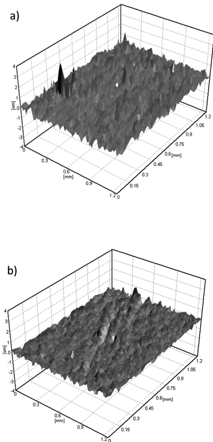
Fig. 8. 3D surface profile of Ni-Mo coatings deposited at different current densities: a) 2.5 A/dm 2 ( R_a = 0.27 \mu\text{m} ) and b) 4 A/dm 2 ( R_a = 0.18 \mu\text{m} )
