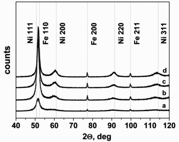
Fig. 9. X-ray diffraction patterns of Ni-Mo alloys electrodeposited at current density: a) 1.5 A/dm 2 (22.2 wt.% Mo), b) 2.5 A/dm 2 (19.0 wt.% Mo), c) 4 A/dm 2 (5.4 wt.% Mo) and d) 5 A/dm 2 (4.9 wt.% Mo)
