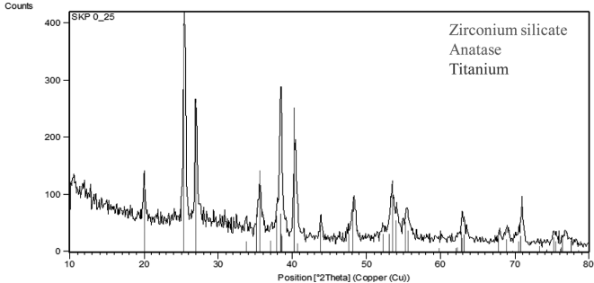
Fig. 3. XRD pattern of sample A2
