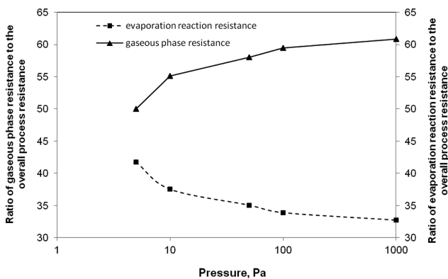
Fig. 8. Ratio of the summary resistance related to mass transfer in the gaseous phase and the act of evaporating to the overall process resistance, depending on pressure
