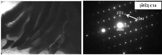
Fig. 3. TEM bright field image and SAED pattern of the \text{Mg}_2\text{Ca} (C14) phase, [-45-12] zone axis
