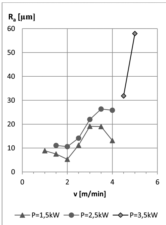
Fig. 16. Dependence of measured average roughness as a function of laser power ( P ) and scanning velocity ( v )
