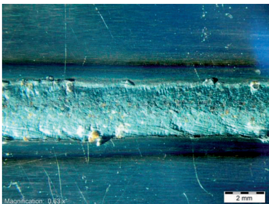
Fig. 3. Typical shape of laser interfusion
