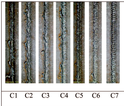
Fig. 6. Vibration-laser interfusions made using Sample No. 3
