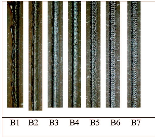
Fig. 5. Vibration-laser interfusions made using Sample No. 2
