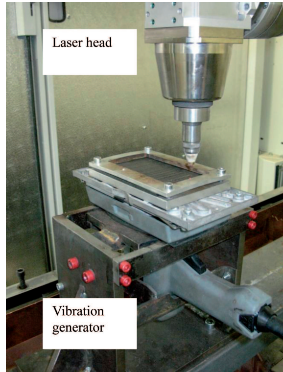
Fig. 1. Vibration-laser stand for melting metal elements
