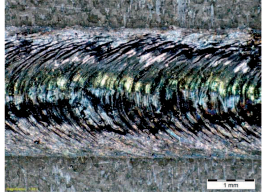
Fig. 7. Front of interfusion No. A1
