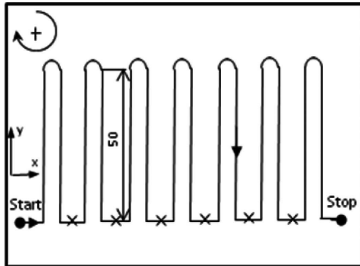
Fig. 2. Diagram showing vibration-laser melting of samples
