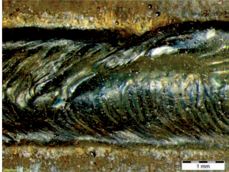
Fig. 10. Front of interfusion No. B1
