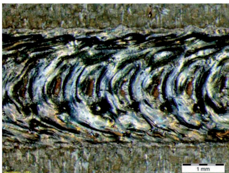
Fig. 12. Front of interfusion No. B7
