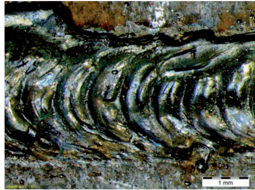
Fig. 14. Front of interfusion No. C4
