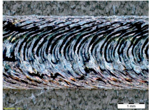
Fig. 8. Front of interfusion No. A4
