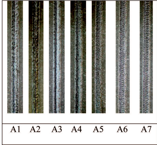
Fig. 4. Vibration-laser interfusions made using Sample No. 1
