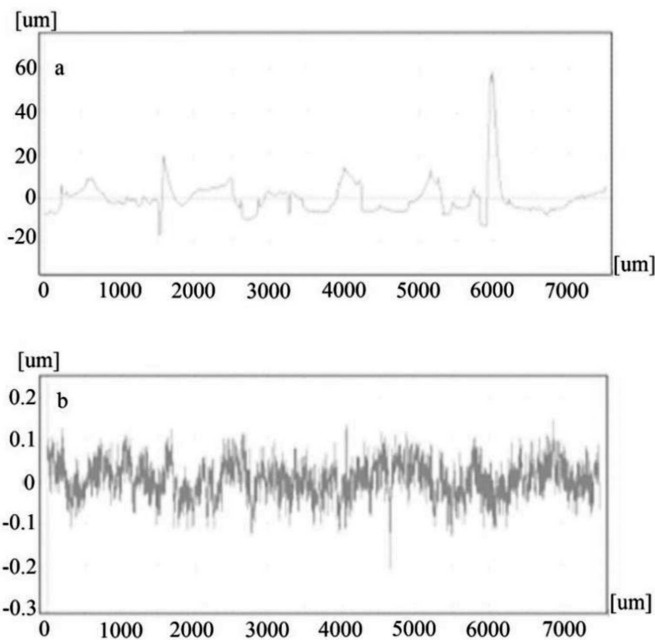
Fig. 9. Examples of measured profiles for chitosan layers deposited in time: (a) 600 s and (b) 30 s
