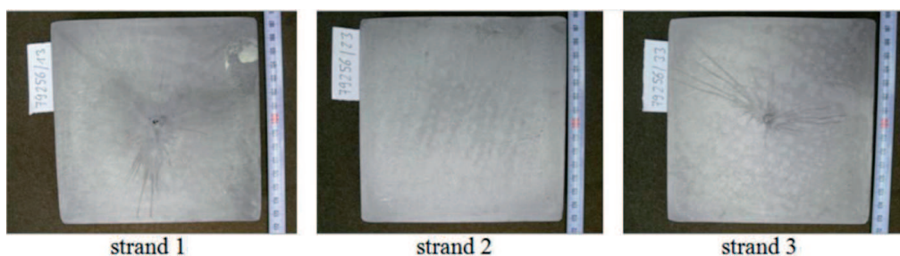
Fig. 8. Macrostructure of ingots' cross-section measuring 140x140 mm, middle of WB1 smelt
