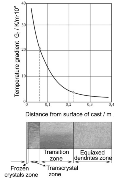
Fig. 2. Impact of the intensity of liquid steel cooling on ingot's structural form
