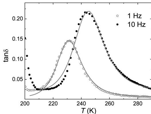
Fig. 5. Thermally activated peak in supercooled PYR 14 -TFSI. The continuous line is a fit according to Eq. (1)
