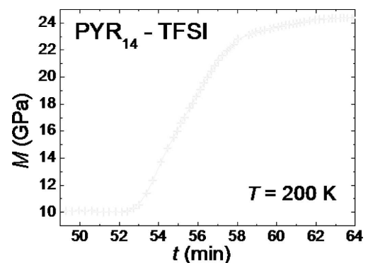
Fig. 6. Isothermal variation of the elastic modulus, measured with the DMA at 200 K, reached on heating, after cooling at 4 K/min down to 150 K
