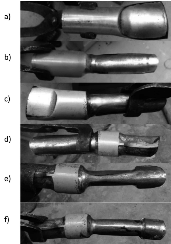
Fig. 12. Subsequent roll passes during rolling of the preform from billet with diameter 042 mm: a) oval - I, b) circle - I, c) oval - II, d) circle - II, e) oval - III, f) circle - III
