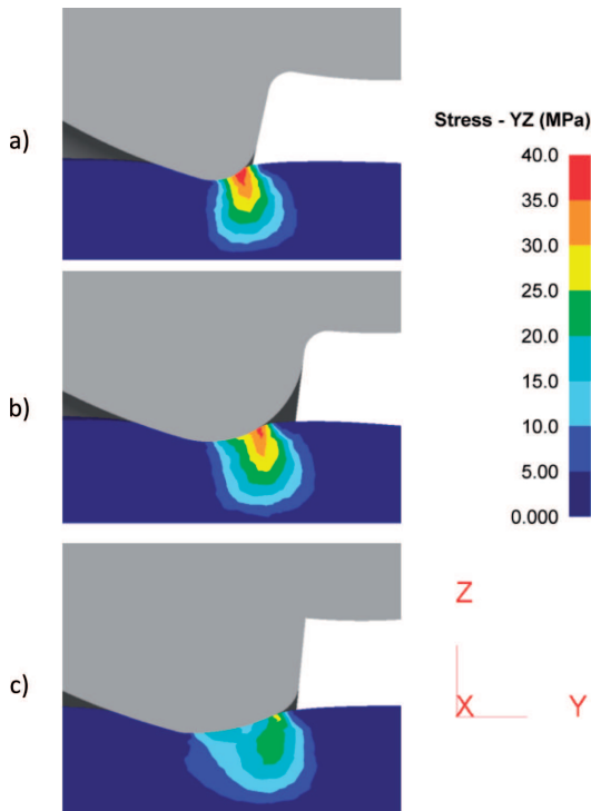
Fig. 7. Shearing stresses distribution at the moment of material clamping by segments: a) segment with radius R = 10 mm, b) R = 20 mm, c) optimized segment
