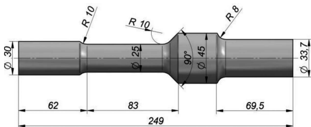
Fig. 1. Shape and dimensions of the lever preform [9]
