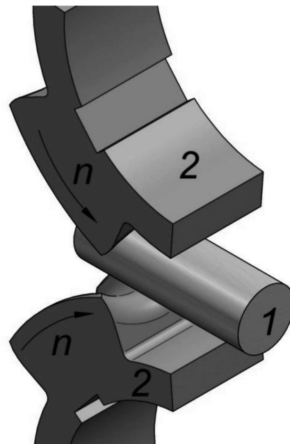
Fig. 2. Geometrical model of the forge rolling process: 1 – billet, 2 – rolling segments
