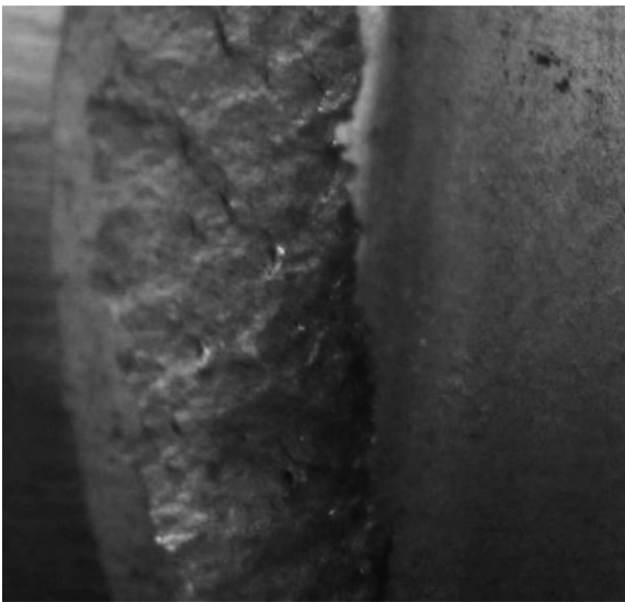
Fig. 4. Photo of the scrap surface obtained during rolling in the oval impression for the roll pass 1
