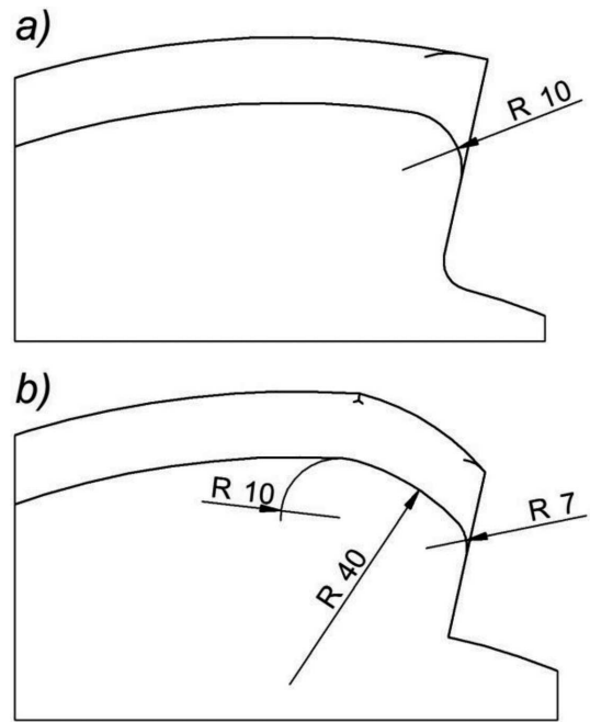
Fig. 5. Tools entrance area for the first roll pass: a) R = 10 mm, b) segment with gradually increasing reduction ratio
