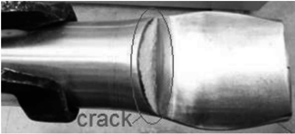
Fig. 3. Crack on the rolled oval for the roll pass 1
