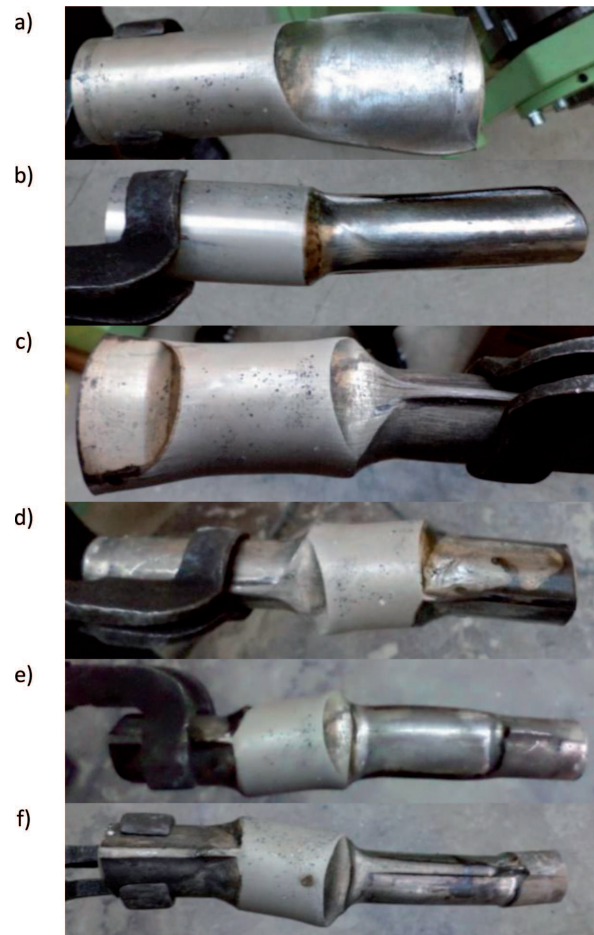
Fig. 11. Subsequent roll passes during rolling of the preform from billet with diameter \varnothing 45 mm: a) oval - I, b) circle - I, c) oval - II, d) circle - II, e) oval - III, f) circle - III
