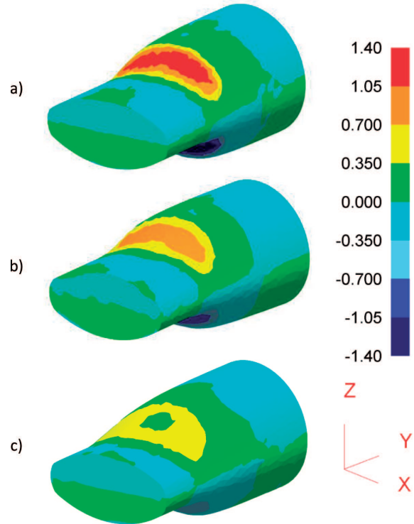
Fig. 8. Non-dilatational strains \gamma_{yz} distribution: a) segment with radius R = 10 mm, b) R = 20 mm, c) optimized segment
