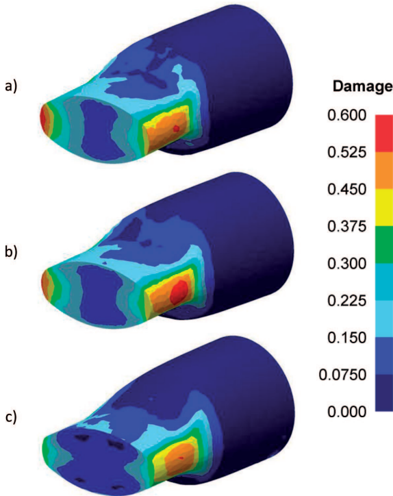
Fig. 6. Distribution of Cockcroft-Latham integral value: a) segment with radius R = 10 mm, b) R = 20 mm, c) segment with gradually increasing reduction ratio
