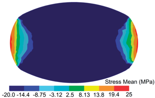
Fig. 9. Mean stresses distribution during rolling in the oval impression for the first roll pass
