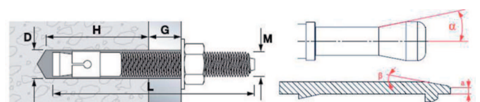
Fig. 9. View of the anchor and its characteristic dimensions
