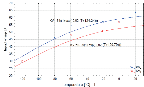
Fig. 4. Impact energy KV of Weldox 1300 steel. KVL – impact energy longitudinal of orientation to rolling direction of KVT – impact energy transverse of orientation to rolling direction
