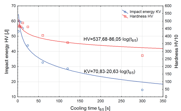
Fig. 5. Impact energy KV and hardness HV of simulated HAZ of Weldox 1300 steel, temperature of the impact test 20°C
