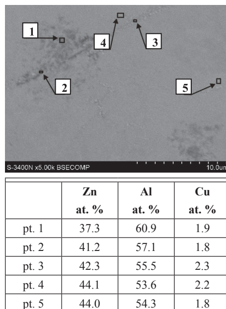
Fig. 1. Structure of the ZnAl40Cu3 alloy after solutionizing 385°C/24h
