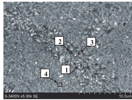
Fig. 4. Structure of the ZnAl40Cu3 alloy after solutionizing 385°C/24h and aging 150°C/24h
