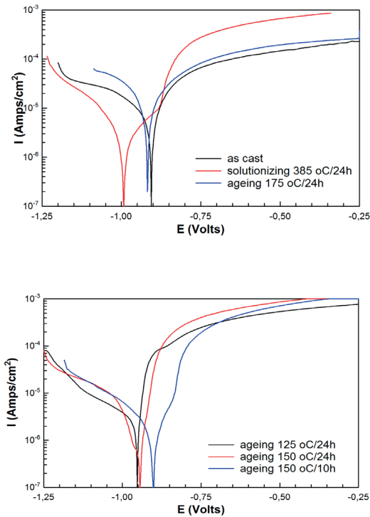
Fig. 6. Potentiodynamic curves of ZnAl40Cu3 alloy after heat treatment in „acid rain”
