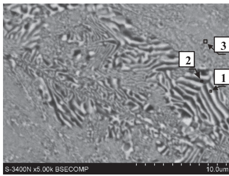
Fig. 2. Structure of the ZnAl40Cu3 alloy after solutionizing 385°C/24h and aging 175°C/24h
