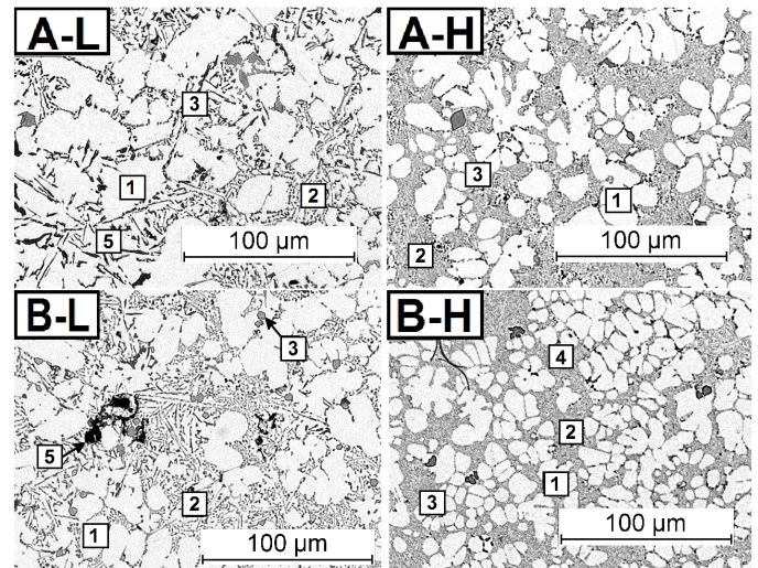
Fig. 6. Microstructures of castings A and B: 1 – phase \alpha , 2 – eutectic mixture, 3 – iron-rich phase, 4 – copper-rich phase, 5 – shrinkage-gas microporosity. Light microscope, magnification: 200 \times , non-etched
