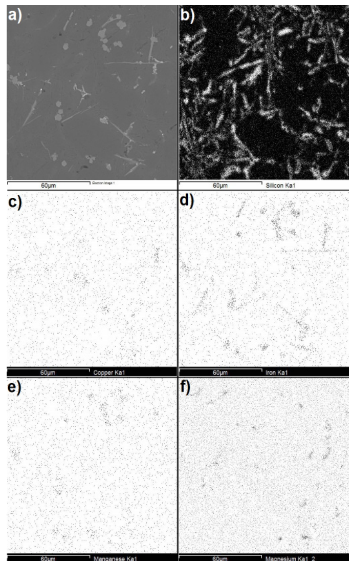
Fig. 9. Distribution of the most important elements in series: C, D, F and G on G-L example: a) SEM image of the structure and the distribution: b) Si, c) Cu, d) Fe, e) Mn, f) Mg; Magnification: 1200×
