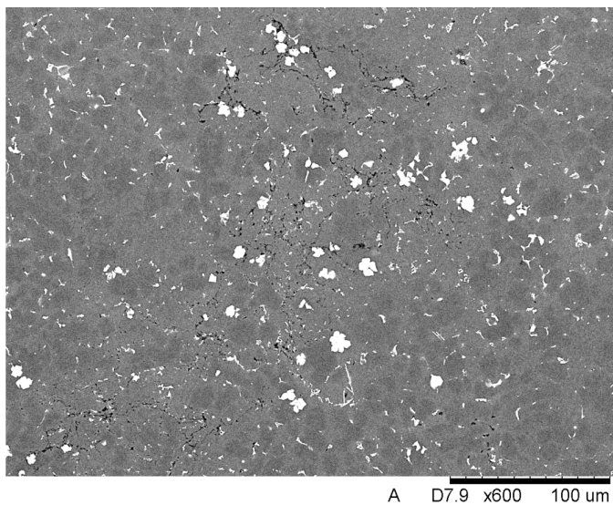
Fig. 5. View of cast F structure with shrinkage-gas microporosity, magnification: 600 \times
