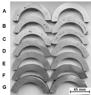
Fig. 2. Specimens in that X-ray examination revealed most numerous internal defects in form of shrinkage cavities and pinholes: lower (L) – left and upper (H) – right
