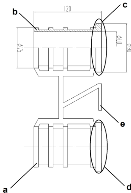
Fig. 1. Lay-out of a mould with shown location of cavities and structure of gating system: a) lower casting (L), b) upper casting (H), c) and d) places of taking samples, e) gating system
