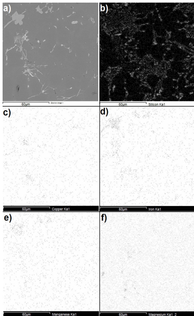
Fig. 8. Distribution of the most important elements in series: A, B and E on A-L example: a) SEM image of the structure and the distribution: b) Si, c) Cu, d) Fe, e) Mn, f) Mg; magnification: 1200×
