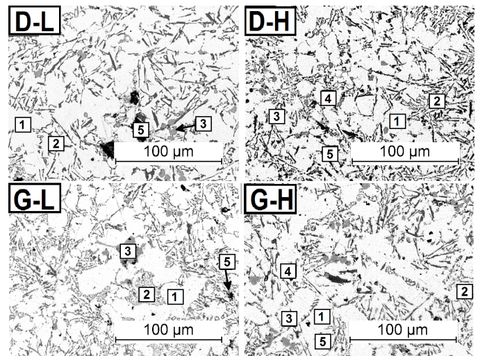
Fig. 7. Microstructures of castings D and G: 1 – phase \alpha , 2 – eutectic mixture, 3 – iron-rich phase, 4 – copper-rich phase, 5 – shrinkage-gas microporosity. Light microscope, magnification: 200 \times , non-etched
