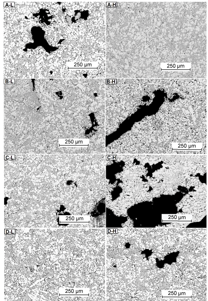
Fig. 3. View of samples' microstructure casts A-D, magnification: 50 \times , non-etched
