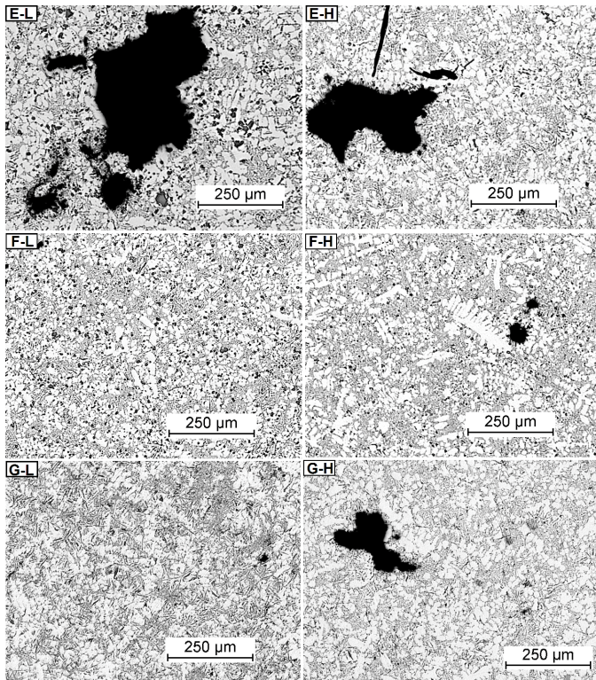
Fig. 4. View of samples' microstructure casts E-G, magnification: 50 \times , non-etched
