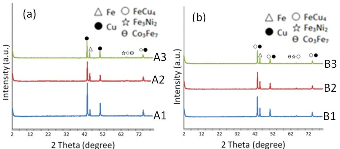
Fig. 6. XRD patterns of a) A samples b) B samples
