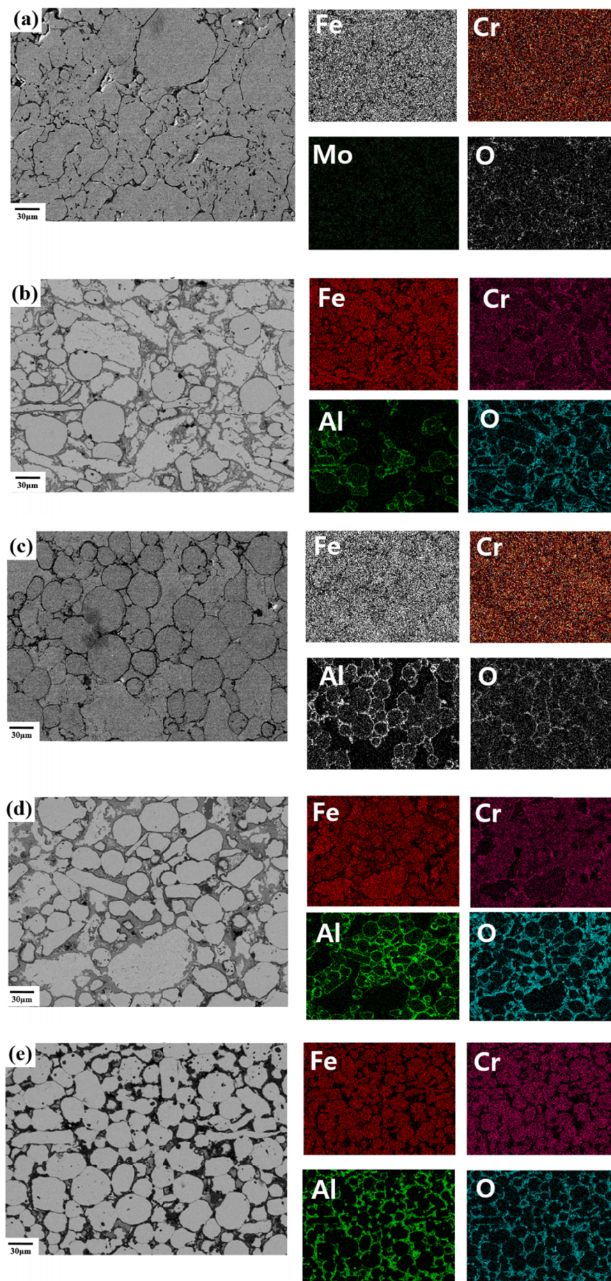
Fig. 5. EDS mapping results of specimens after 210hr exposure at 950°C in air: (a) 434L, (b) 434L (0.75) + Feccraloy (0.25), (c) 434L (0.5) + Feccraloy(0.5), (d) 434L (0.25) + Feccraloy (0.75) and (e) Feccraloy
