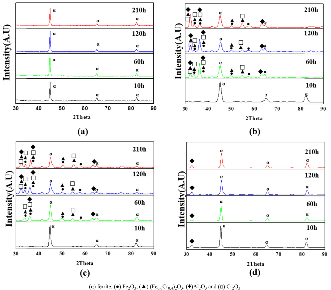
Fig. 4. X-ray diffractograms corresponding to respective specimens after different periods of exposure at 950^\circ\text{C} in air: (a) 434L, (b) 434L (0.75) + Feclloy (0.25), (c) 434L (0.25) + Feclloy (0.75) and (d) Feclloy
