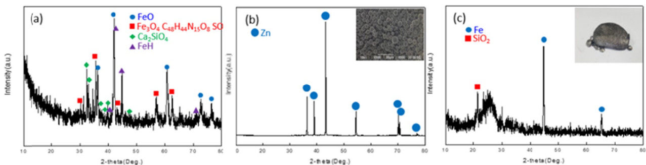
Fig. 1. 1 XRD Patterns of each specimen ((a)Steelmaking dust treated DRI raw material (b) Recovered zinc dust (c) Produced pig iron)
