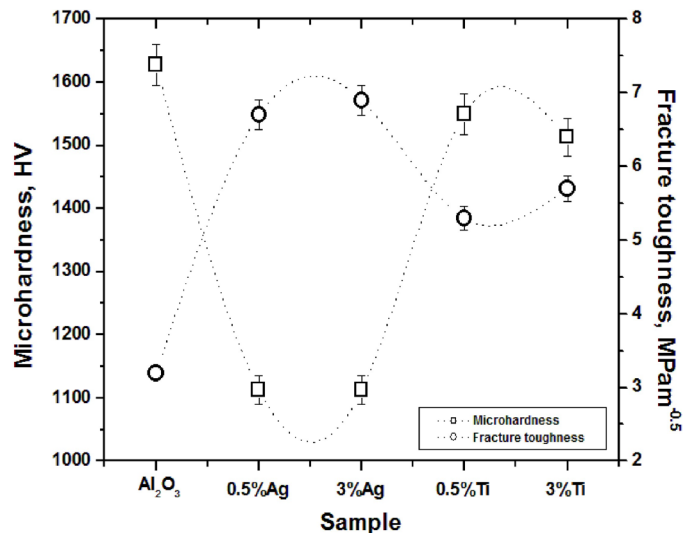
Fig. 8. Hardness and fracture toughness of sintered samples
