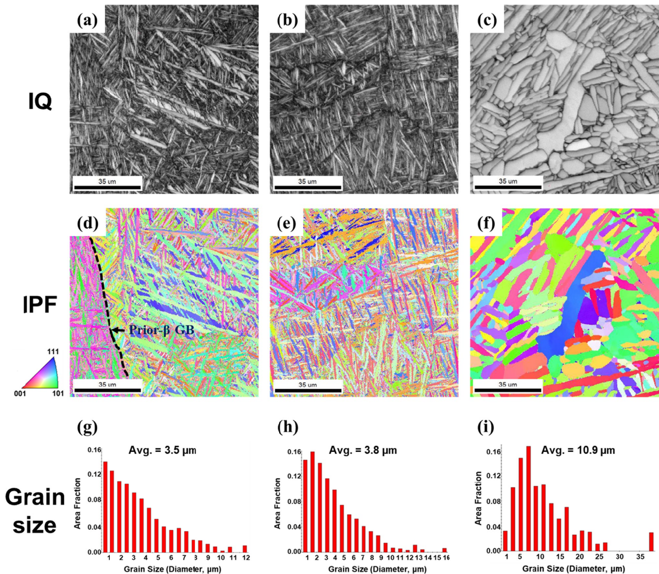
Fig. 2. EBSD observations exhibiting with IQ, IPF maps and grain size distribution of SLMed Ti-6Al-4V alloy after different heat treatments including (a, d, g) SLMed, (b, e, h) annealing and (c, f, i) HIP
