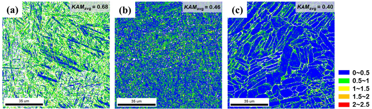
Fig. 3. EBSD KAM maps of SLMed Ti-6Al-4V alloy after different heat treatments including (a) SLMed, (b) annealing and (c) HIP
