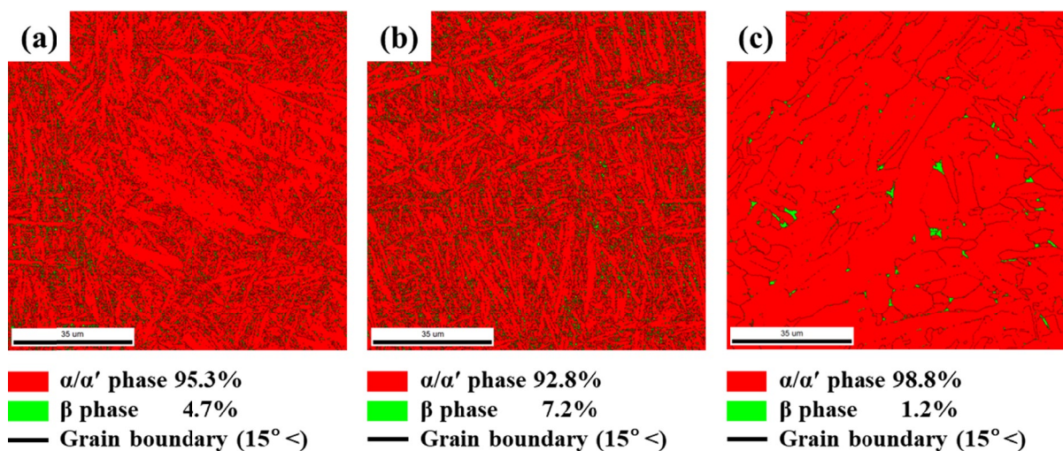
Fig. 1. EBSD observations exhibit the distribution of grain boundaries and phase maps of SLMed Ti-6Al-4V alloy after different heat treatments including (a) SLMed, (b) annealing and (c) HIP
