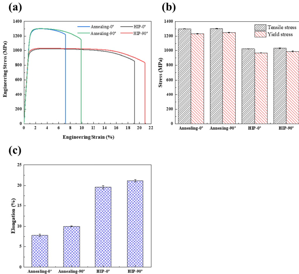
Fig. 4. Tensile properties of the annealing and HIP samples with different building direction (a) Engineering stress-strain curves, (b) Summary of the UTS, YS, (c) Summary of the Elongation
