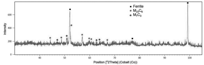
Fig. 4. XRD analysis of the investigated alloy
