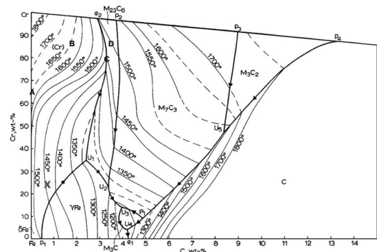
Fig. 6. Liquidus projection for the Fe-Cr-C ternary system [26÷29]
