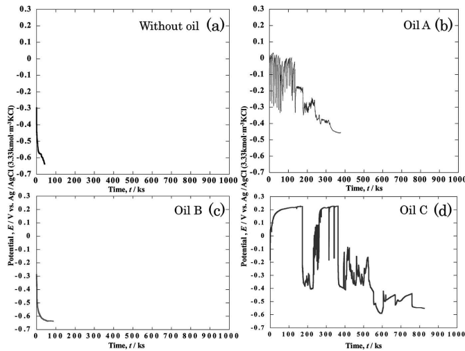
Fig. 3. Corrosion potential of sintered Fe-Cu-C alloy measured in thin corrosive solution (a) without oil, (b) coated with Oil A, (c) coated with Oil B and (d) coated with Oil C
