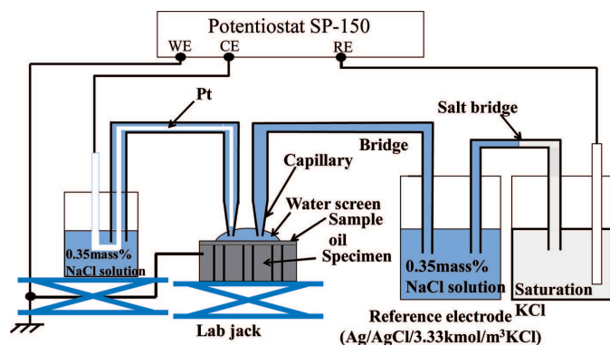
Fig. 1. Schematic diagram of apparatus for the polarization curve measured
