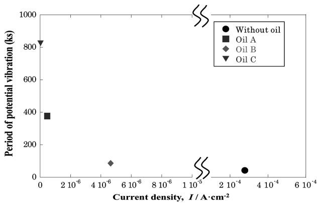
Fig. 4. Negative correlation between corrosion rate and period of potential oscillation
