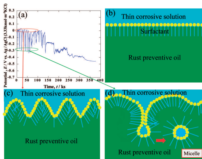
Fig. 2. (a) Corrosion potential of sintered Fe-Cu-C alloy measured with oil A in thin corrosive solution[10] and schematic diagram of formation micelle: (b) the initial stage, (c) the second stage, (d) the third stage
