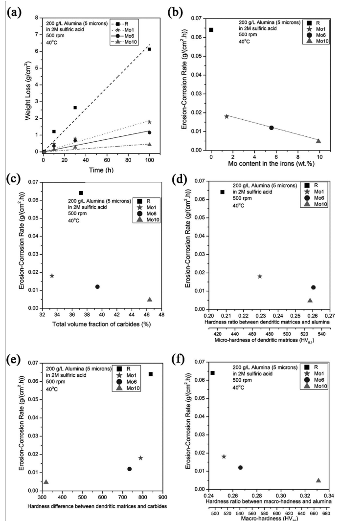
Fig. 3. (a) weight loss after erosion-corrosion testing as a function of testing time, (b to f) plots of wear rate versus the Mo content (wt.%), the total volume fraction of carbides, the micro-hardness of dendritic matrices, the hardness difference between dendritic matrices and carbides, and the macro-hardness of the irons, respectively
