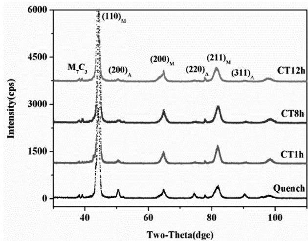
Fig. 1. X-ray diffraction patterns of the commercial high carbon alloyed tool steel after quenching and different CT soaking time at -130°C
