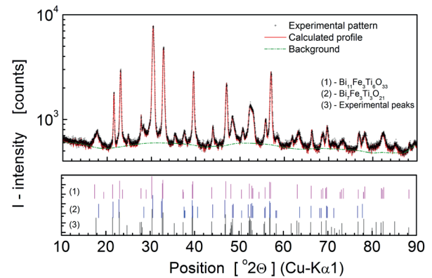
Fig. 2. X-ray diffraction matching parameters for \text{Bi}_6\text{Fe}_2\text{Ti}_3\text{O}_{18} ceramics fabricated via solid state reaction route and pressureless sintering at T=850^\circ\text{C} ; (bottom plot – peak positions of the experimental pattern and the main reference phases)
