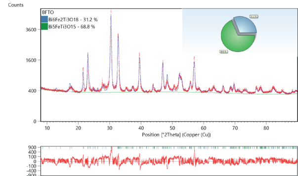
Fig. 4. X-ray diffraction pattern after refinement of the elementary cell parameters for BFTO ceramics sintered at T=850^\circ\text{C} in assumption of the multiphase sample; bottom plot shows the difference between the experimental (dots) and refined (solid line) diffraction patterns
