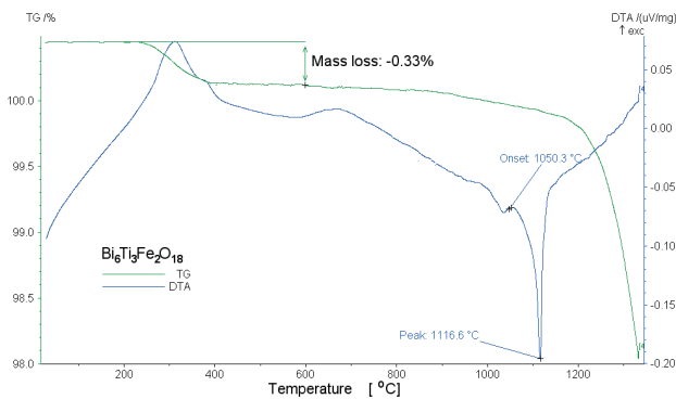
Fig. 1. Results of thermal analysis of stoichiometric mixture of oxides forming \text{Bi}_6\text{Fe}_2\text{Ti}_3\text{O}_{18}
