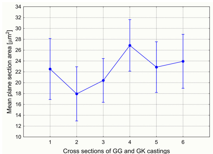
Fig. 14. Comparison of mean plane section area of (\gamma + \gamma') eutectic areas between the cross sections of GK and GG cast jointly
