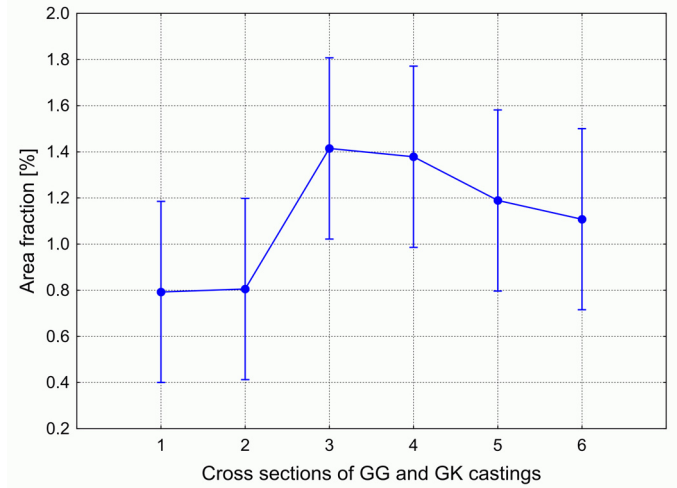
Fig. 10. Comparison of area fraction of (\gamma + \gamma') eutectic areas between the cross sections of GK and GG cast jointly
