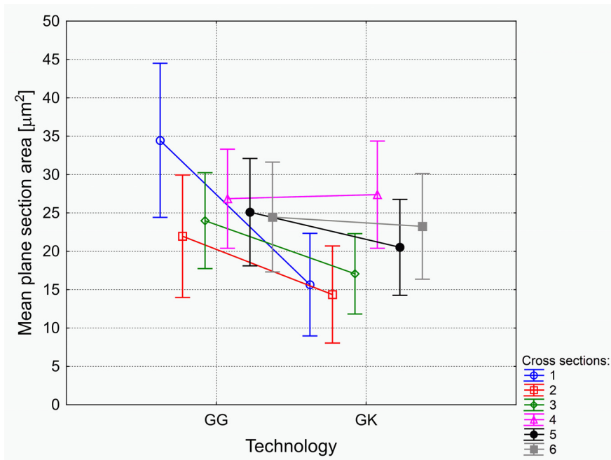
Fig. 16. Comparison of both technologies and the six cross sections of GK and GG casts in regard to mean plane section area of (γ + γ') eutectic areas between
