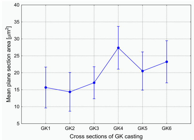
Fig. 12. Comparison of mean plane section area of (\gamma + \gamma') eutectic areas on the cross sections of GK cast
