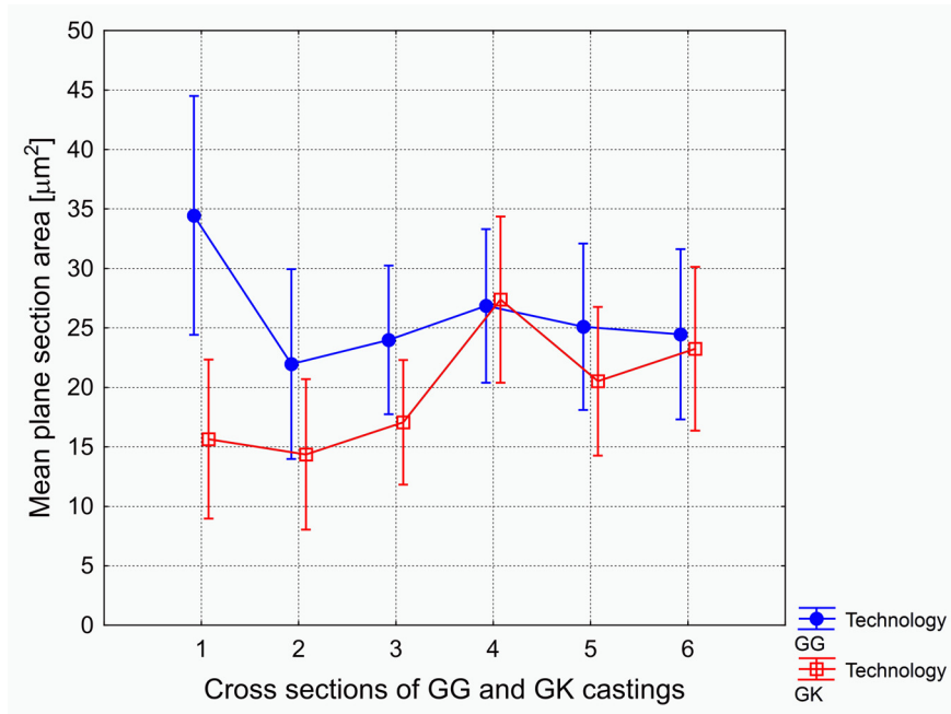
Fig. 15. Comparison of both technologies with the cross sections of GK and GG cast jointly in regard to mean plane section area of (γ + γ') eutectic areas
