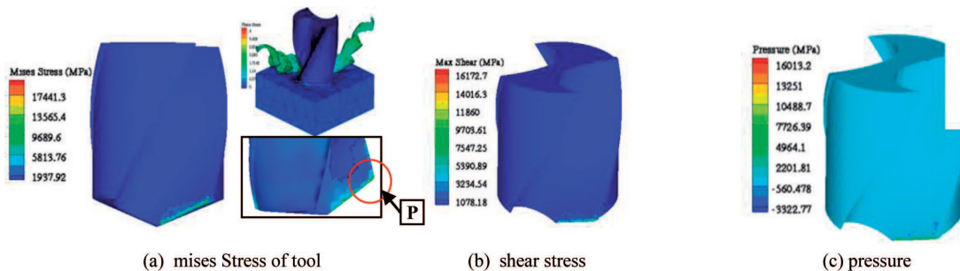
Fig. 5. Stress and pressure during cutting operation
