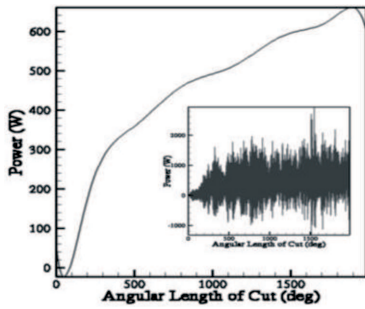
Fig. 8. Cutting power
