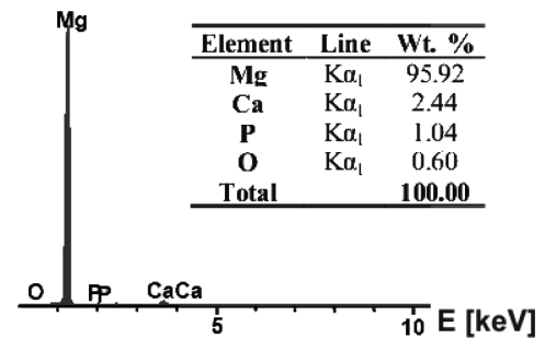
Fig. 2. EDS surface spectrum of the bulk Mg-10 wt.% HA sample
