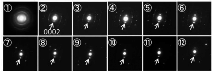
Fig. 3. A series of SAED patterns obtained from each area of spheroidal graphite marked by (1) - (12) in Fig. 2
