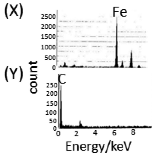
Fig. 4. EDS profiles obtained for areas marked by X and Y in Fig. 2
