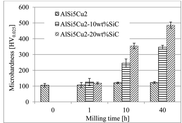
Fig. 7. Microhardness as function of milling time for 0, 10 and 20wt% SiC
