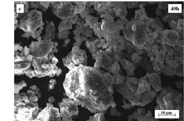
Fig. 3. (a – c) SEM micrographs of composite powders of composition AlSi5Cu2+20wt%SiC after different milling time
