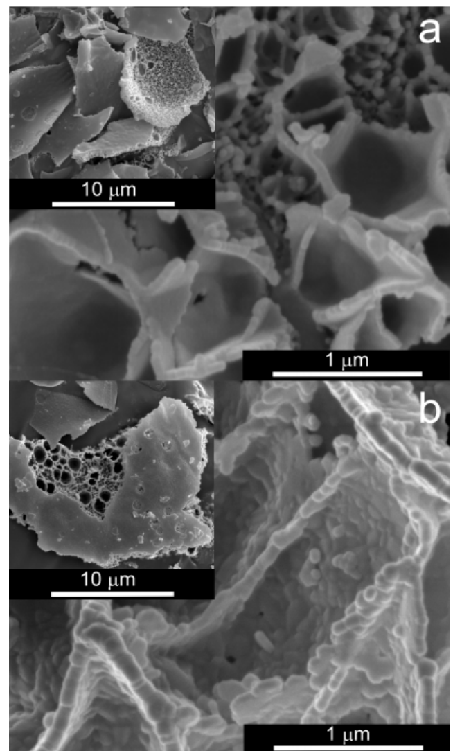
Fig. 7. Micrographs of yttria nanopowder obtained by SCS reaction with citric acid calcined at temperature of: a) 800^\circ C and b) 1100^\circ C
