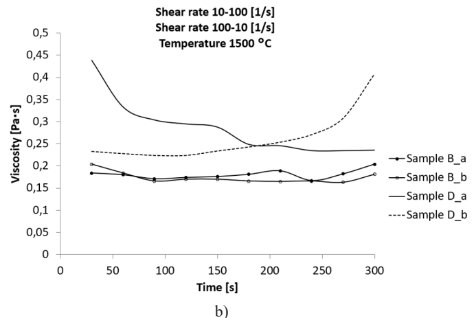
Fig. 12. Changes in the dynamic viscosity coefficient values of analysed slag systems in time for changeable shear rate values 10\text{-}100 \text{ s}^{-1} and 100\text{-}10 \text{ s}^{-1} for a) sample A and C; b) sample B and D
