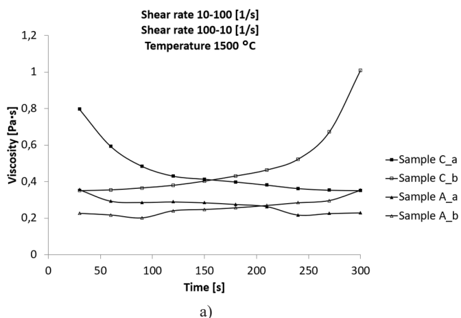
Fig. 12. Changes in the dynamic viscosity coefficient values of analysed slag systems in time for changeable shear rate values 10\text{-}100 \text{ s}^{-1} and 100\text{-}10 \text{ s}^{-1} for a) sample A and C; b) sample B and D
