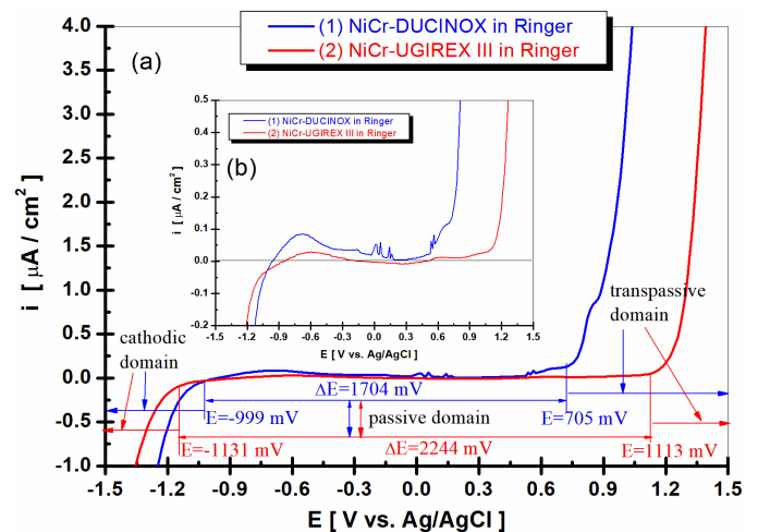
Fig. 6. Potentiodynamic polarization diagrams recorded in Ringer biological solution recorded at a scan rate of 5 \text{ mV/s} for: (1) Ni-Cr alloy Ducinox; (2) Ni-Cr alloy Ugirex III
