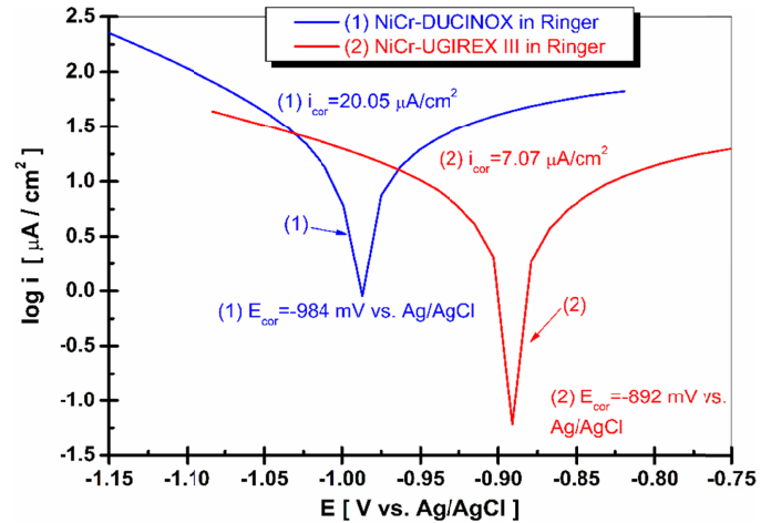
Fig. 3. Linear polarization diagrams recorded in Ringer solution with a scan rate of 1 mV/s for Ni-Cr alloy: (1) Ni-Cr alloy Ducinox; (2) Ni-Cr alloy Ugirex III
