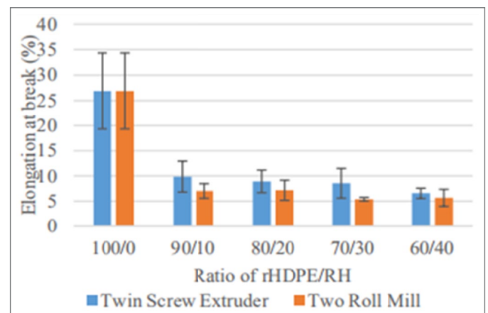
Fig. 2. Elongation at break of r-HDPE/RH composites
