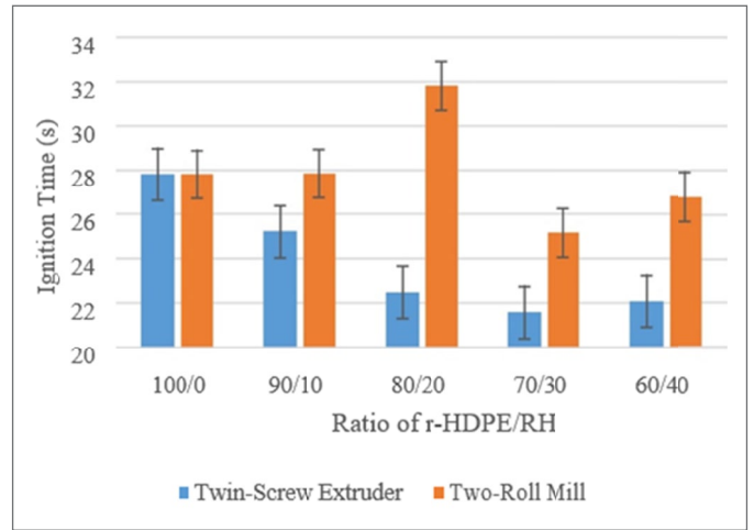
Fig. 5. Ignition time of r-HDPE/RH composites
