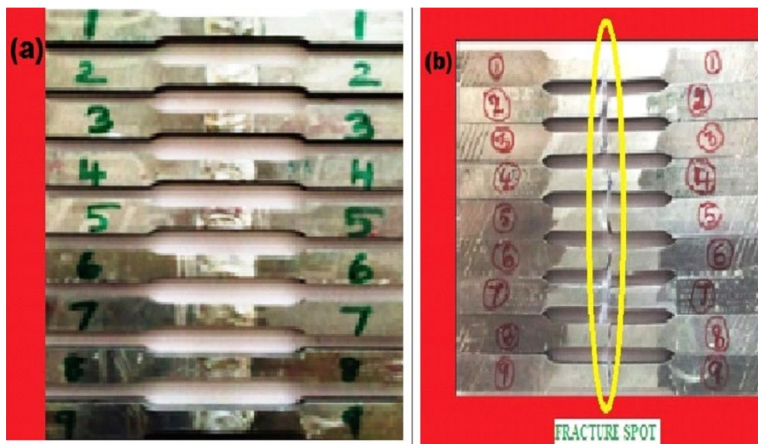
Fig. 3. (a) Tensile test specimens before tensile test; (b) Fractured tensile specimens after test
