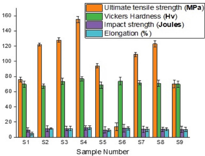
Fig. 5. Experimental results – Mechanical Properties of TIG welded joints
