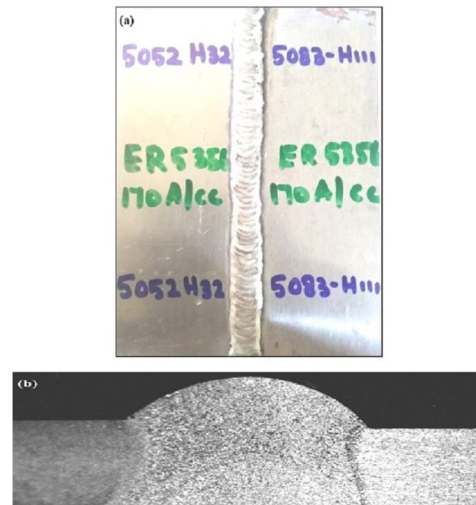
Fig. 9. (a) TIG welded AA5052-H32 – AA5083-H111 under optimized process parameters (b) Macrostructure of the TIG welded joint
