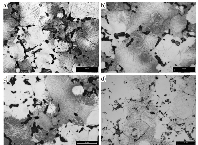
Fig. 5. Microstructures of Ti-5553 alloy induction sintered at the temperature of 1300°C and time of a) 112,5 b) 225 s, c) 375,5 s, d) 450 s
