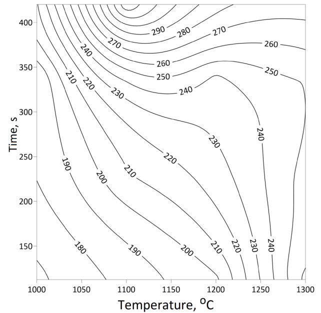
Fig. 6. Map of sample average hardness as a function of sintering temperature and time
