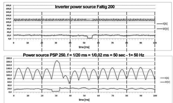
Fig. 4. Examples of real current signals (blue colour) and voltage (red colour). The current waveform for the inverter power source is clearly more consolidated (narrower range of variability) if compared to signals obtained for conventional source
