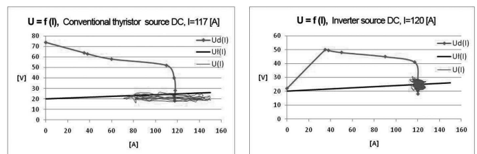
Fig. 2. The example of static real characteristics of the welding power source U_d(I) Conventional arc characteristic U_f=20+0,04I , real arc operation U(I) , Welding power source: conventional thyristor rectifier and inverter equipment. Electrode: E 380 R 11, \phi 3,2 \times 350 mm
