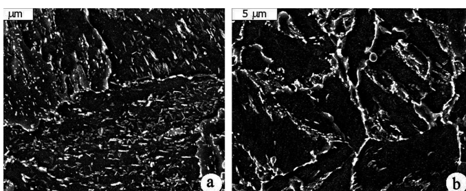
Fig. 2. The microstructure a – non-modified, b – modified, SEM
