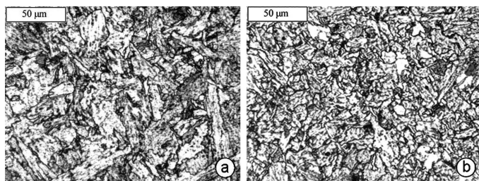
Fig. 1. The microstructure: a – non-modified, b – modified, LM
