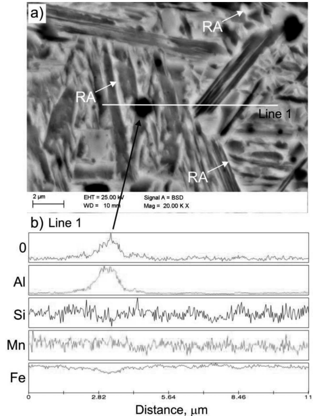
Fig. 7. Non-metallic inclusions in the FZ composed of martensitic-bainitic laths and interlath retained austenite RA (a) and linear distribution of the content of individual elements along line 1 (b)
