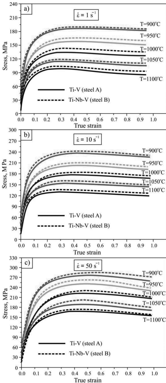
Fig. 2. Influence of the plastic deformation temperature and strain rate (a-c) on a shape of \sigma - \epsilon curves for investigated steels
