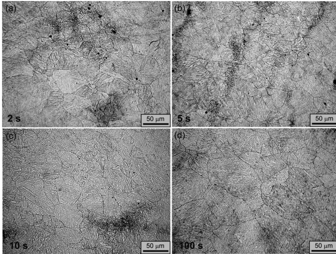
Fig. 4. Prior austenite grains of steel B revealed after two-stage compression test at the temperature of 1000°C at the rate of 10 s -1 applying breaks between deformation steps in a range from 2 to 100 s (a-d)
