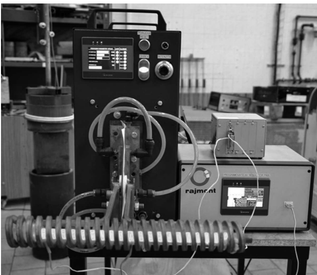
Fig. 2. Induction heat treatment
