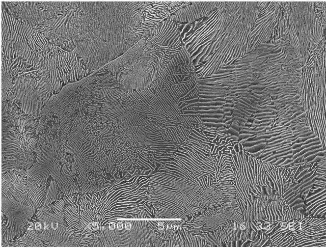
Fig. 1. Microstructure of initial state of 100CrMnSi6-4 steel – hardness 383 HV10
