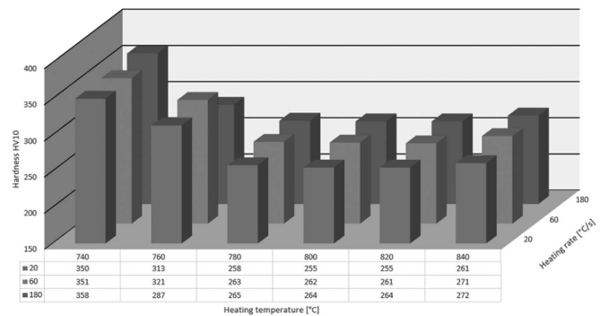
Fig. 9. HV10 hardness achieved with individual schedules
