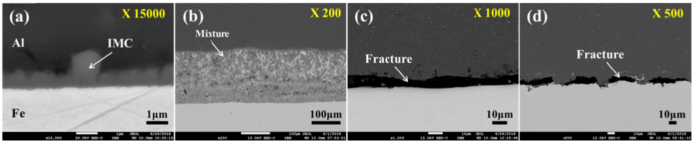
Fig. 3. Cross-sectional SEM micrograph of the bonded specimen for each surface-treated steel; (a) Galvanized steel-10 μm (#1), (b) Galvanized steel-100 μm (#2), (c) Galvannealed steel (#3), (d) Zn thermal spray coating (#4)
