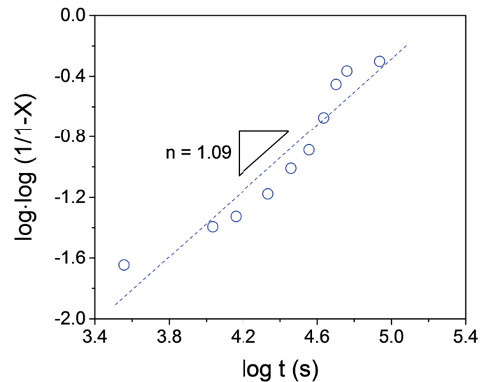
Fig. 4. Change in \log \cdot \log(1/1-X) with \log t at 428 K in AZ91 alloy
