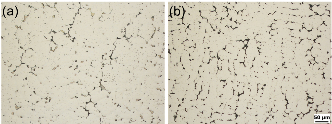
Fig. 1. Optical microstructures of as-cast alloys. (a) Al-7 mass%Mg and (b) Al-7 mass%Mg-1 mass%Cu alloys
