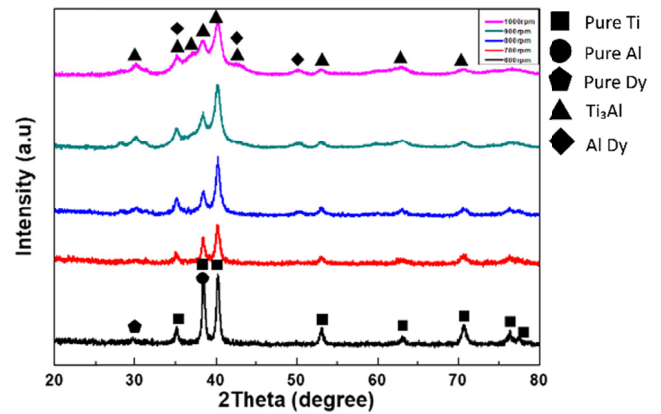
Fig. 5. XRD patterns of as milled powders
