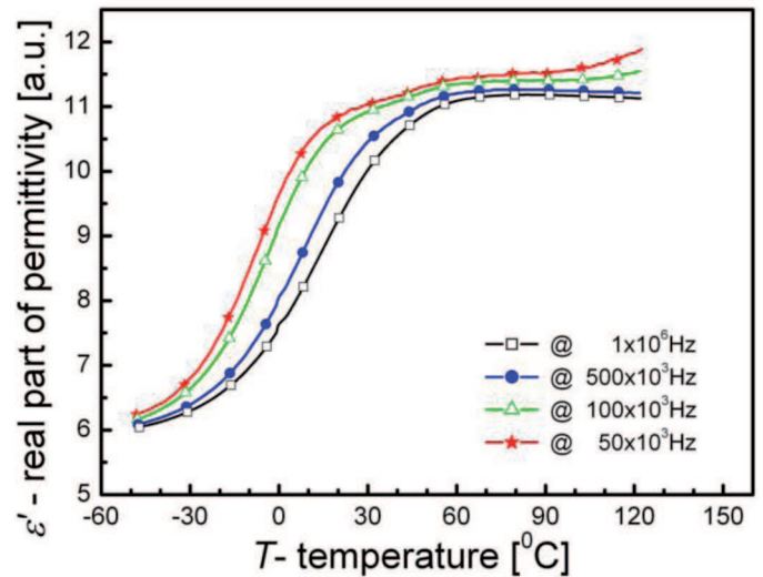
Fig. 10a. Temperature dependence of the real part of dielectric permittivity \epsilon' for polyvinylidene fluoride PVDF
