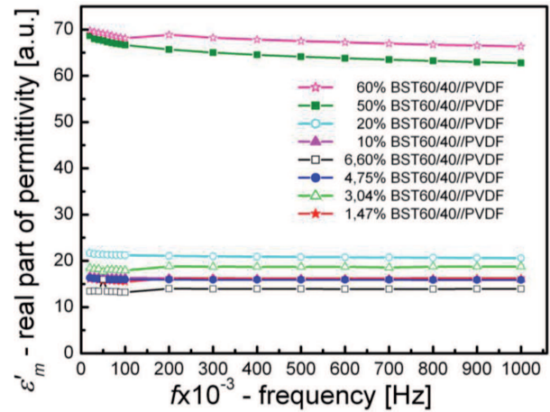
Fig. 12. Frequency dependence of the maximum value of \epsilon'_m for different content of the ceramic phase for BST60/40/PVDF composites
