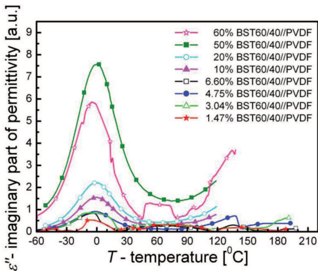
Fig. 11b. Temperature dependence of the imaginary part of dielectric permittivity \epsilon'' for BST60/40/PVDF composites at f=100\text{kHz}
