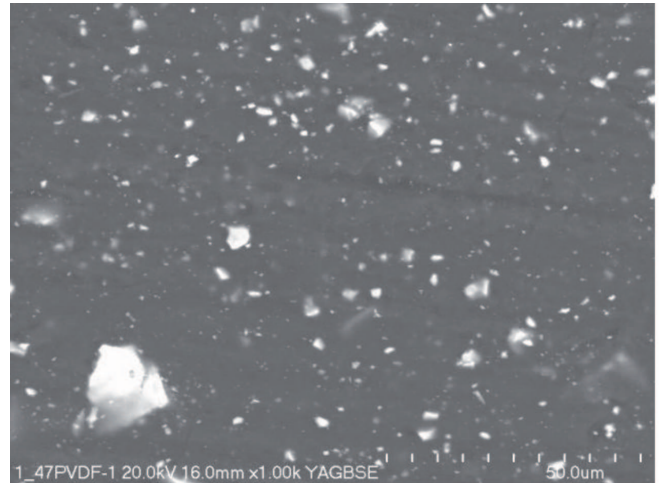
Fig. 2b. SEM micrograph of 1.47%BST60/40/PVDF composite
