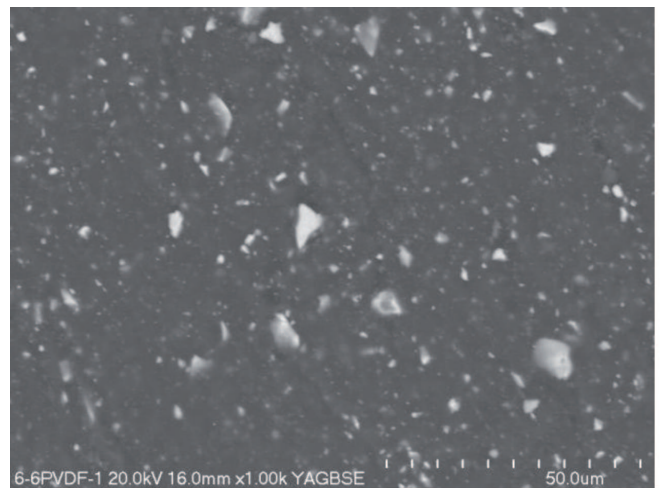
Fig. 3b. SEM micrograph of 6.6%BST60/40/PVDF composite
