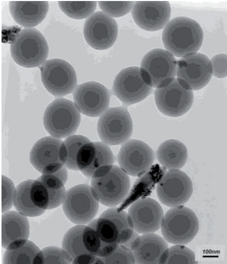
Fig. 2a. TEM micrograph of 1.47%BST60/40/PVDF composite
