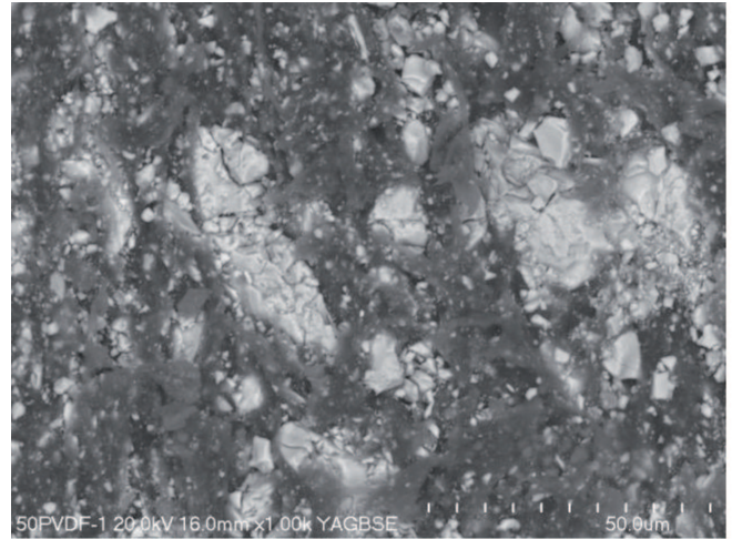
Fig. 5b. SEM micrograph of 50%BST60/40//PVDF composite
