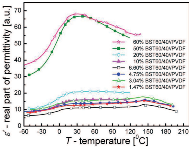
Fig. 11a. Temperature dependence of the real part of dielectric permittivity \epsilon' for BST60/40/PVDF composites at f=100\text{kHz}
