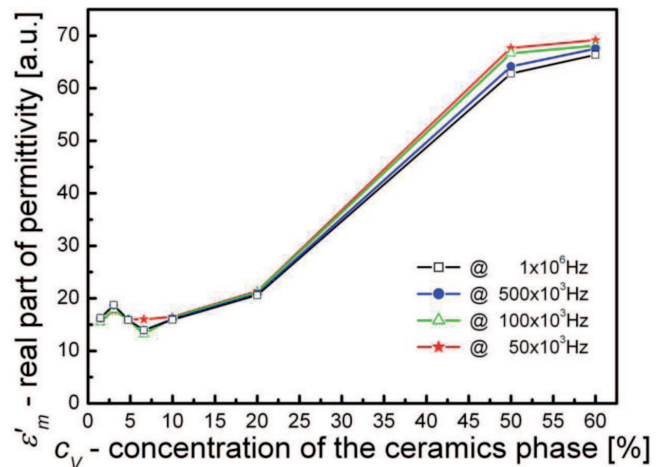
Fig.13. Dependence of the real part of dielectric permittivity \epsilon'_m on the volume fraction of ceramic phase for BST60/40/PVDF composite at f=50\text{kHz} , f=100\text{kHz} , f=500\text{kHz} , f=1\text{MHz}
