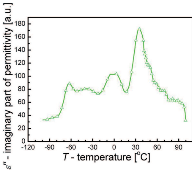
Fig. 9b. Temperature dependence of imaginary part of dielectric permittivity \epsilon'' for BST60/40 ceramic at f=100\text{kHz}
