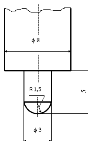
Fig. 8. Sample used in laboratory wear tests
