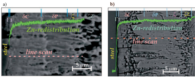
Fig. 1. The varying Zn – solute redistribution in the (Zn) – coating obtained: a/ for 100 [s] of a dipping; the S235 steel substrate, b/ for 60 [s] of a dipping; the S355 steel substrate; (EDS technique); (the chemical concentration of both steels is delivered within the caption to Fig. 1 in Ref. [26])
