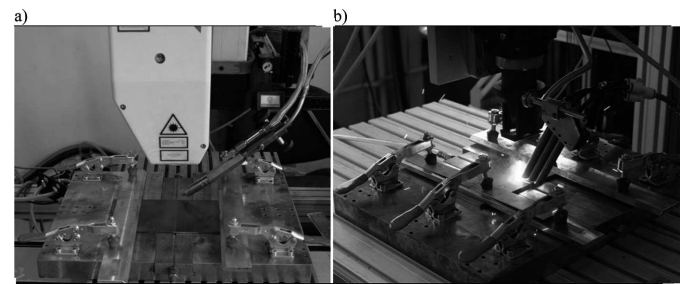
Fig. 1. Experimental setup for autogenous laser welding of butt joints equipped with : a) HPDDL ROFIN DL 020, and b) Disk laser TRUMPF TruDisk 3302
