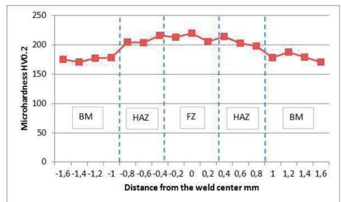
Fig. 9. Microhardness distribution on the cross-section of butt joint welded by the Disk laser at heat input of 38 J/mm, ( t_{8/5} = 0.16\text{ s}</math>), Table 5
